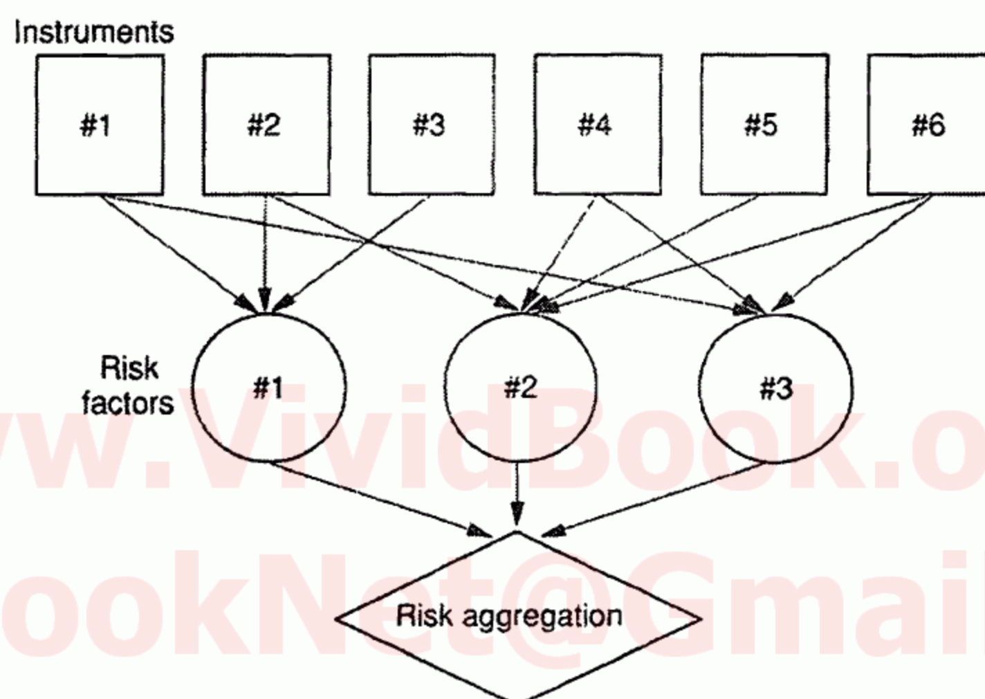
FIGURE 16.1 Mapping Approach
