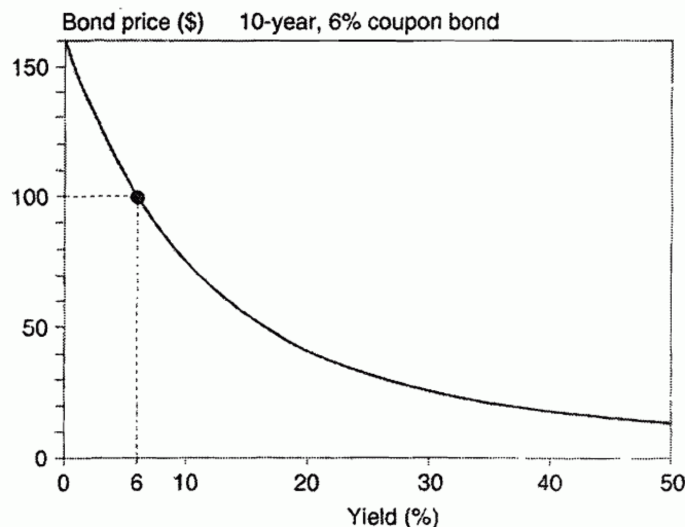
FIGURE 6.1 Price-Yield Relationship
