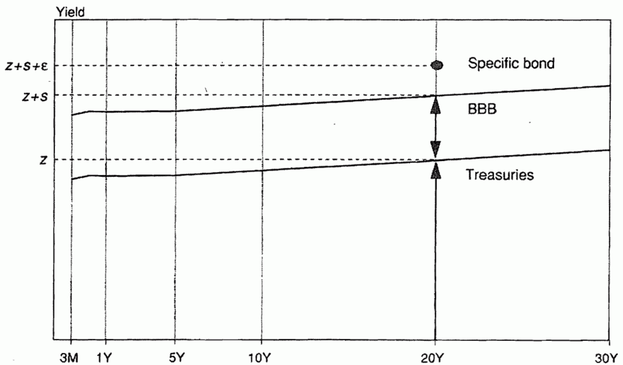
FIGURE 16.2 Yield Decomposition
