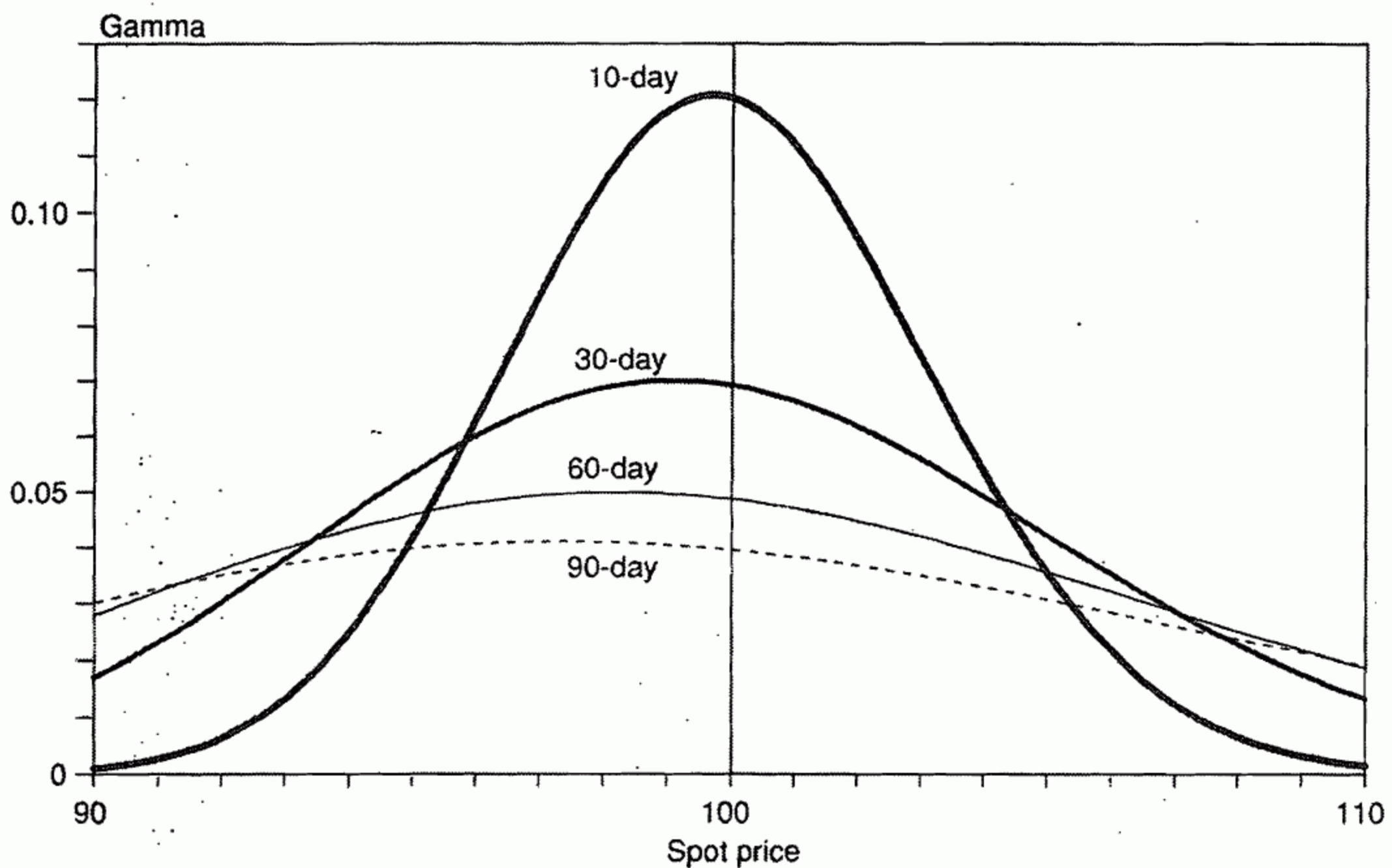
FIGURE 14.3 Option Gamma
