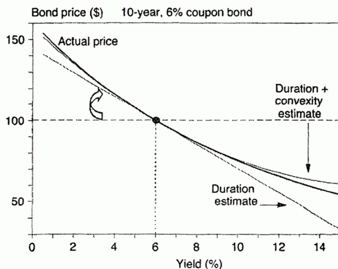
FIGURE 6.2 Price Approximation
