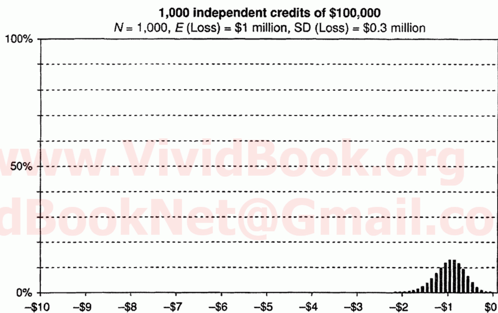
FIGURE 19.3 (Continued)
