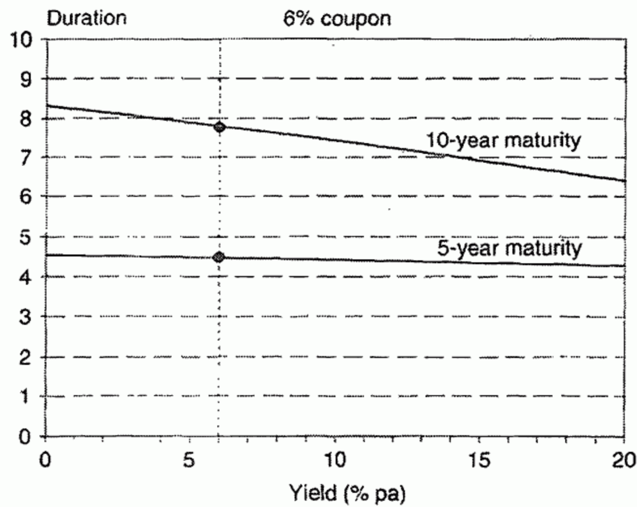
FIGURE 6.7 Duration-Yield Relationship
